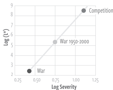
Fig 6. Log L^* versus q .
