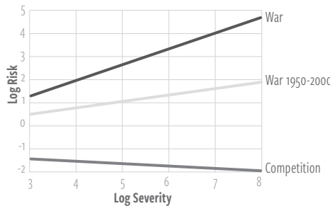
Fig 2. Log Risk versus Log Severity s for three q values.
