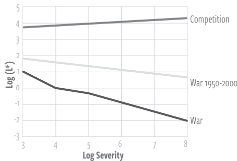
Fig 4. Log critical likelihood ratio L^* versus log severity s for three q values and where \bar{C}/C=270/(s \times 18.6s^{-q}) .
