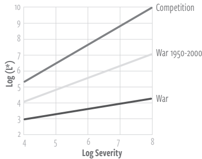
Fig 5. Log L^* versus log severity s for three q values and \bar{C}/C=1 .
